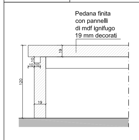
PART. 1 finitura pedana
