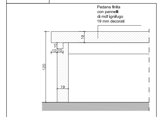
PART. 2 finitura pedana
